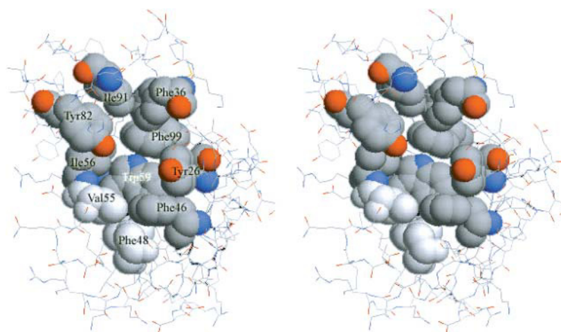
FIGURE 1 Stereo view of the binding pocket of FKBP12 formed by the hydrophobic residues Ile91, Phe36, Phe99, Tyr26, Phe46, Phe48, Val55, Ile56, Tyr82, and Trp59.
